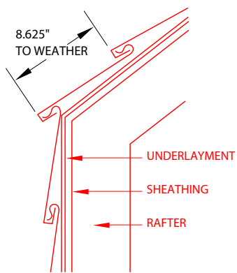
GAMBREL DETAIL
